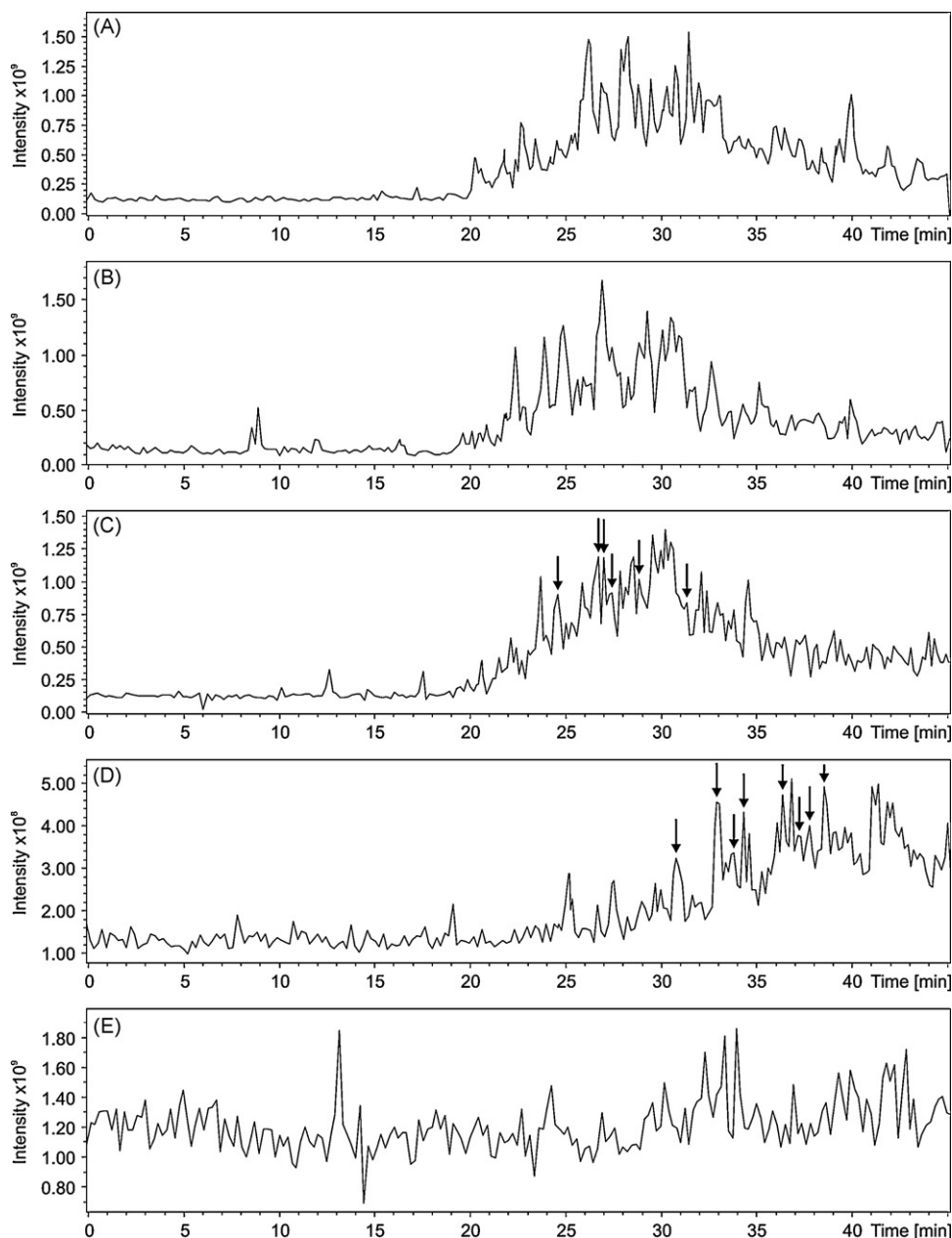
Fig. 4. CE/ESI-MS tryptic peptide maps of BSA: (A) control sample, BSA modified by (B) glucose, (C) ribose, (D) glyoxal, (E) glutardialdehyde (arrows indicate CML-modified peptides). For details see Section 2.
