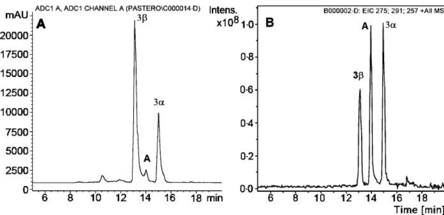
Figure 5 Conversion of androstanolone by chicken 20HSD. (A) Sample (radioactivity detection); (B) standards (MS detection). 3 \beta , 5 \alpha -androstan-3 \beta ,17 \beta -diol; A, 5 \alpha -androstan-17 \beta -ol-3-one; 3 \alpha , 5 \alpha -androstan-3 \alpha ,17 \beta -diol.
